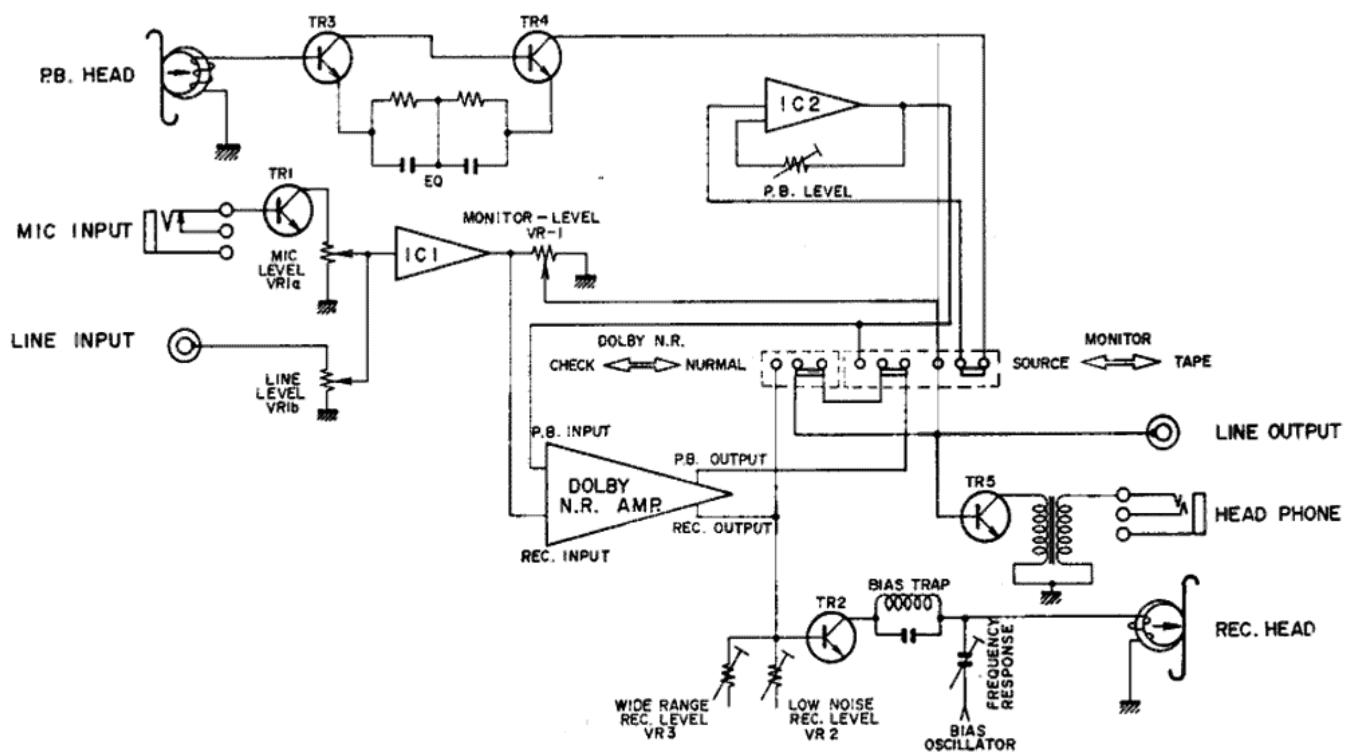
Fig. 18 AMP. SYSTEM BLOCK DIAGRAM
