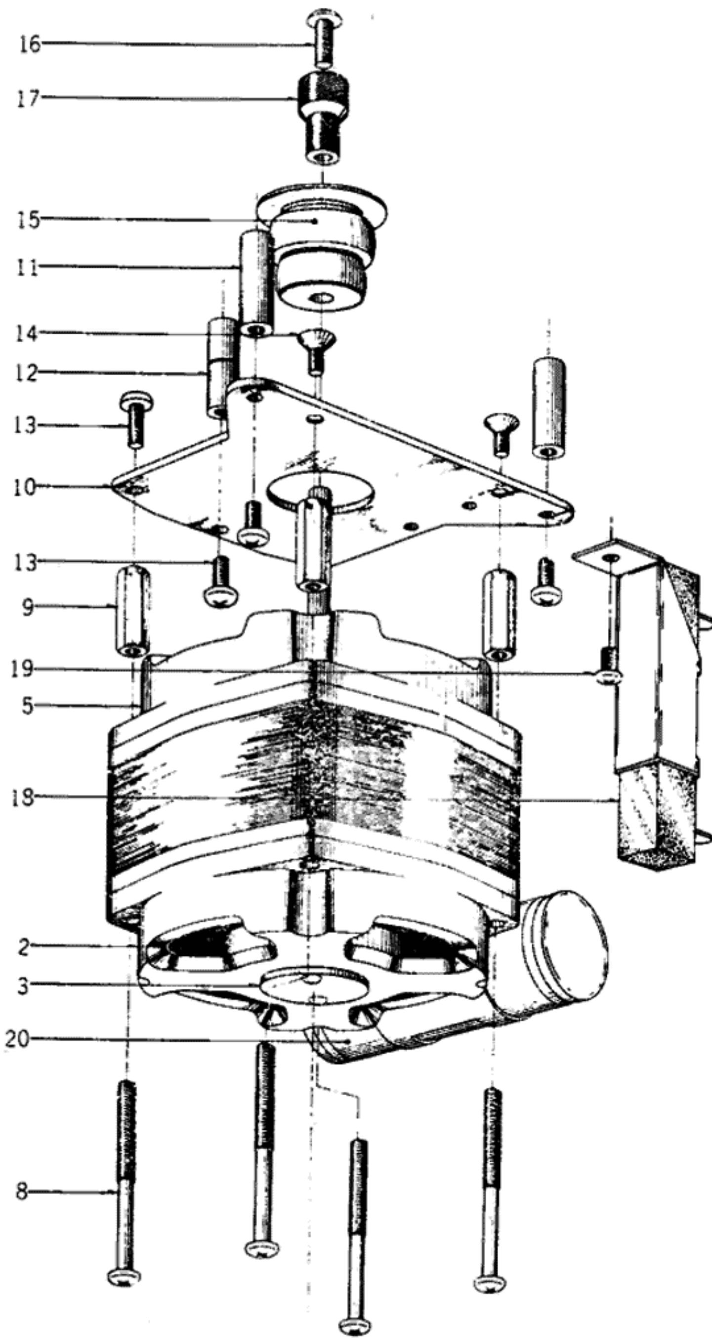
FIG. 3 ILLUSTRATION OF MOTOR BLOCK
