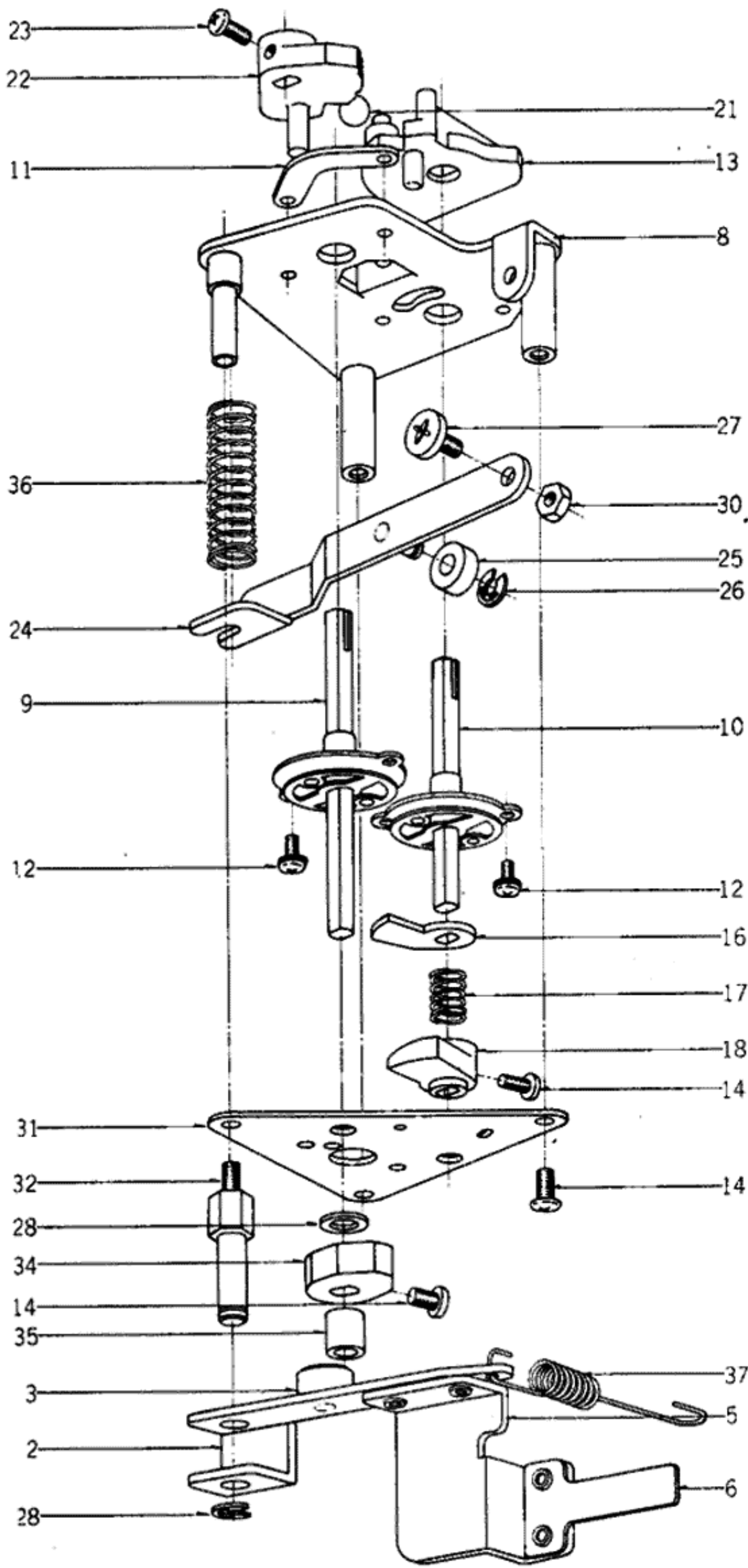
FIG. 5 ILLUSTRATION OF SWITCH BLOCK
